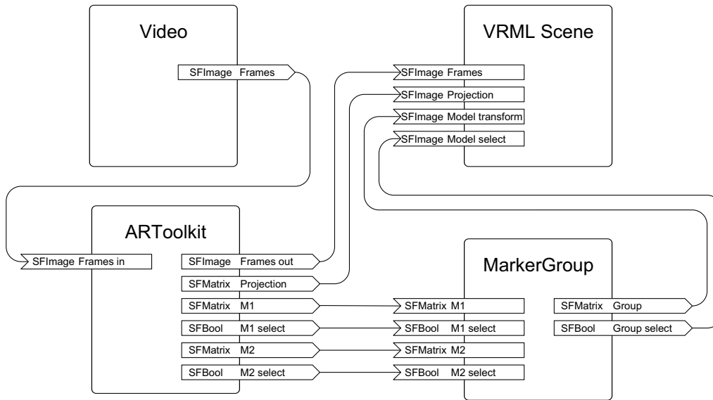
Figure 7: Data flow graph for example application.
