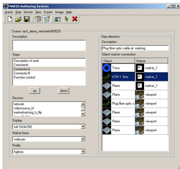
Figure 3: Example authoring application for step-by-step guide applications.
